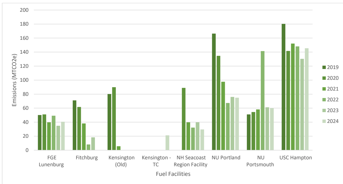
Figure 2: Total annual emissions from fuel consumption across all Unitil facilities
