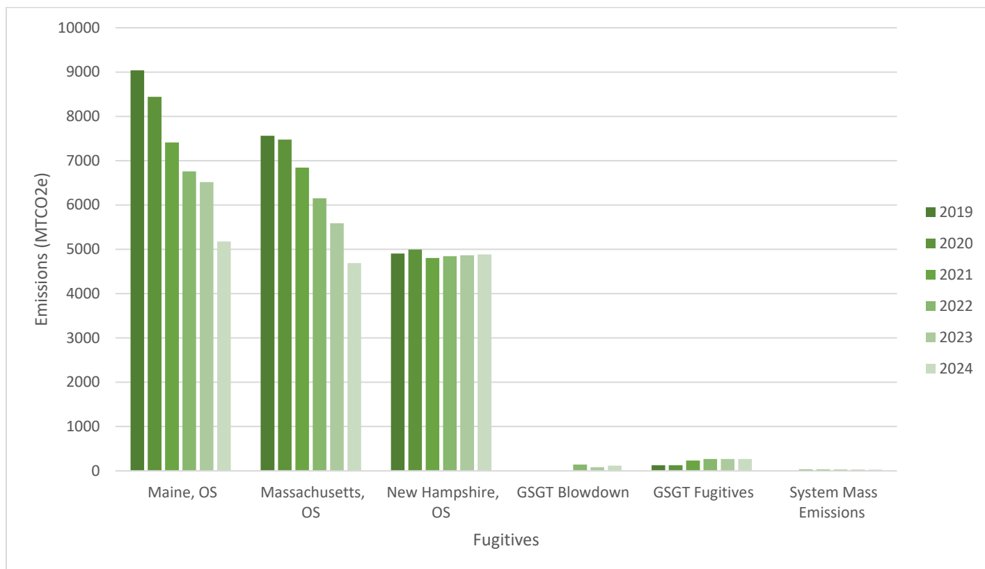
Figure 3: Total annual emissions from fugitives across all operational states and from transmission and distribution
