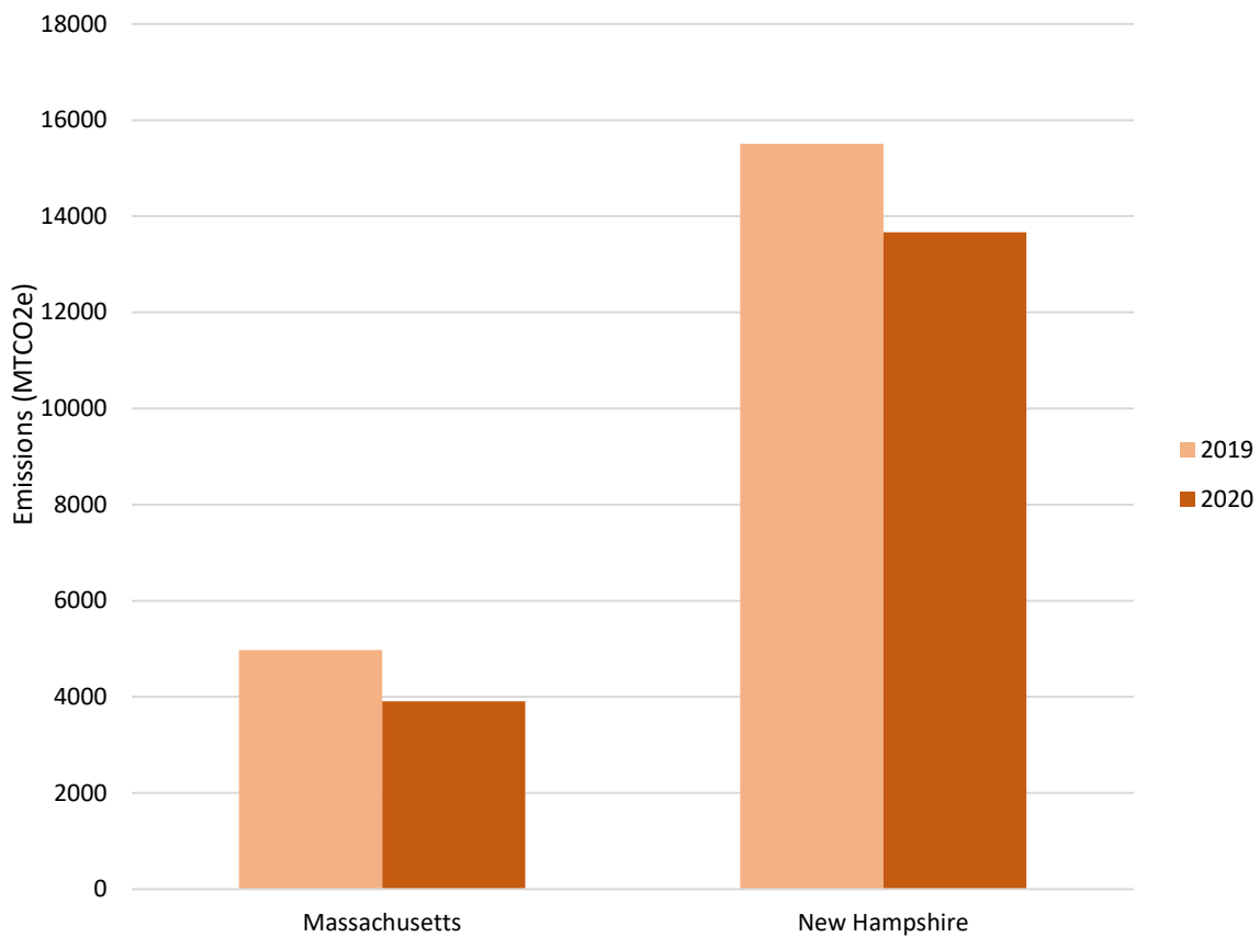
Figure 8: 2019-2020 Emissions from Transmission and Distribution Losses
