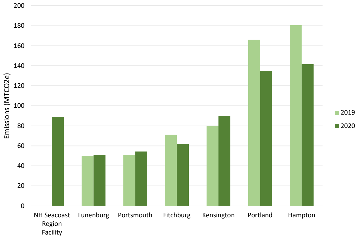
Figure 1: 2019-2020 Emissions from Fuel Use at Company Buildings
