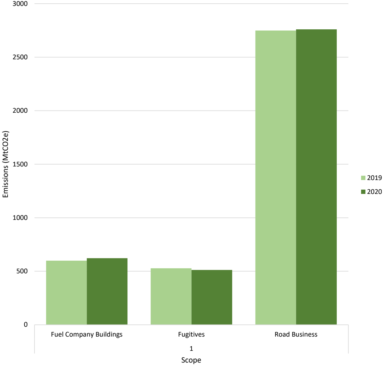
Figure 2: 2019-2020 Scope 1 Summary Chart
