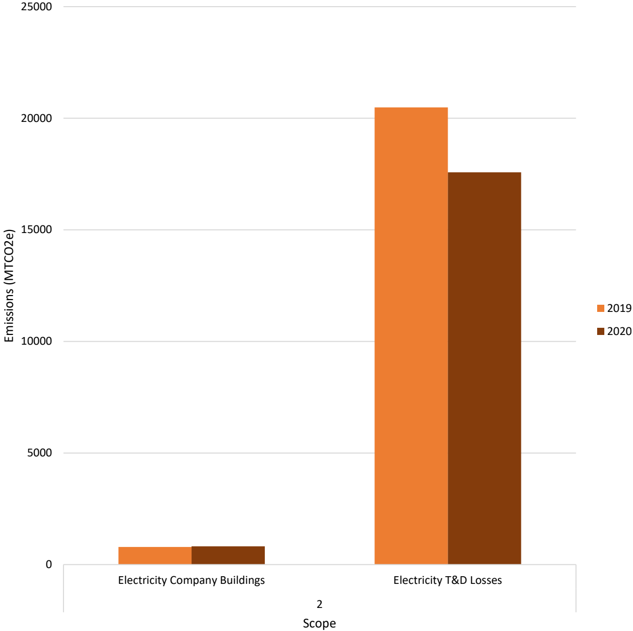
Figure 6: 2019-2020 Scope 2 Summary Chart
