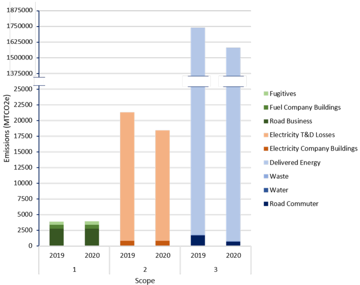
Figure 1: 2019-2020 Emissions by Scope and Category
