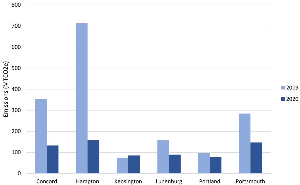
Figure 13: 2019-2020 Emissions from Commuting
