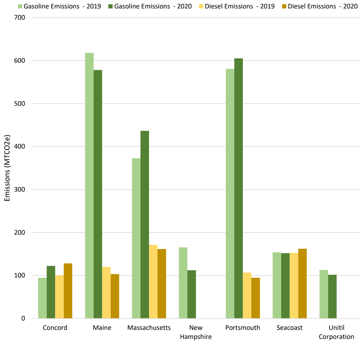
Figure 5: 2019-2020 Emissions from Road Business
