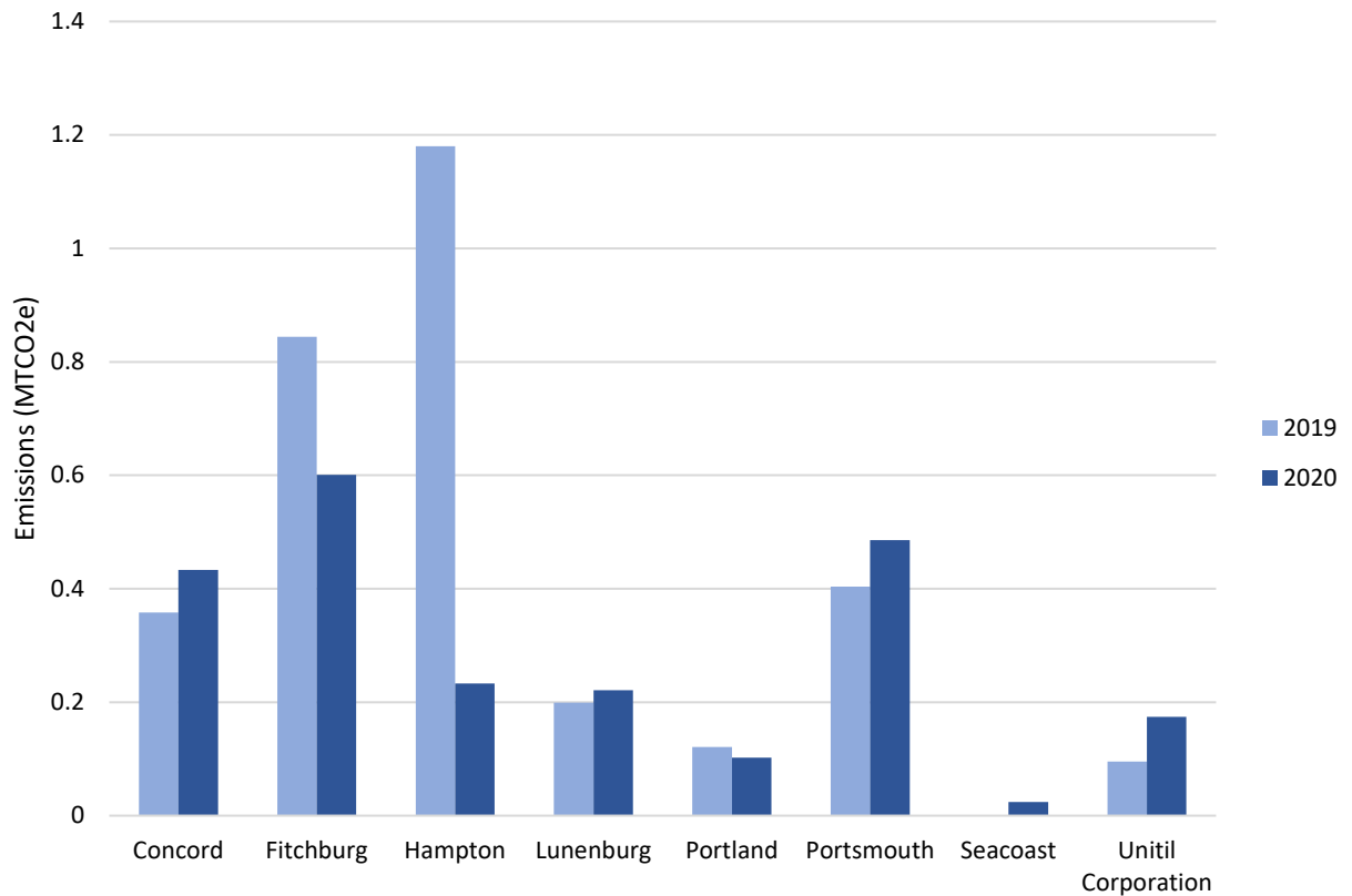
Figure 11: 2019-2020 Emissions from Water
