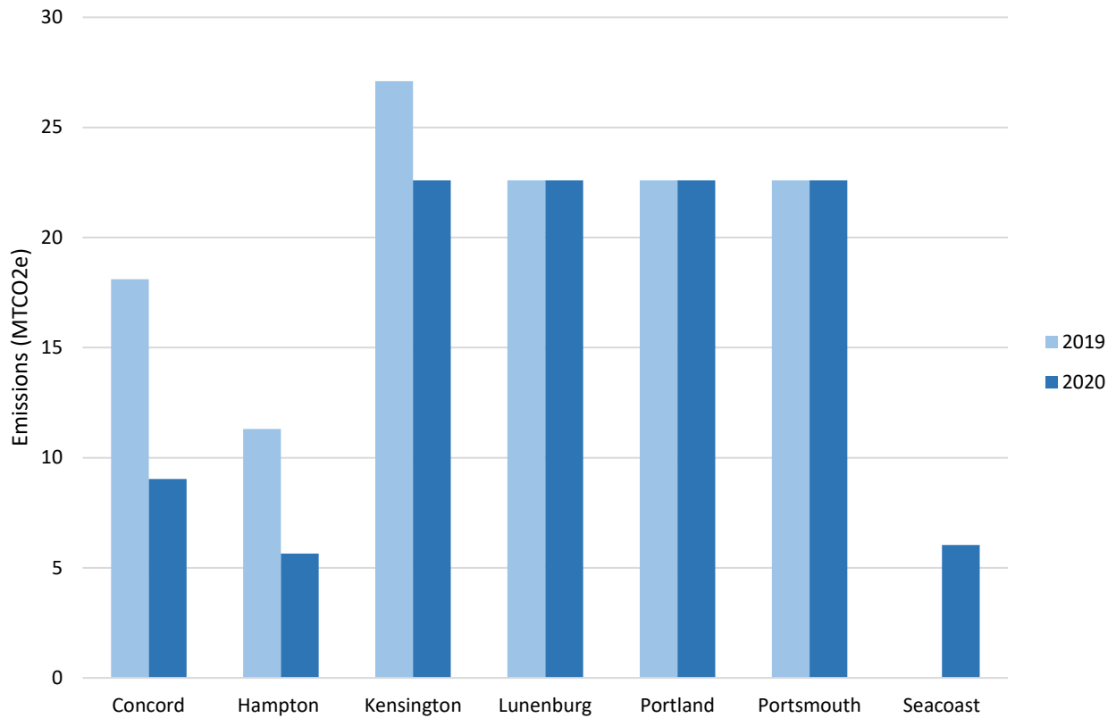
Figure 10: 2019-2020 Emissions from Waste
