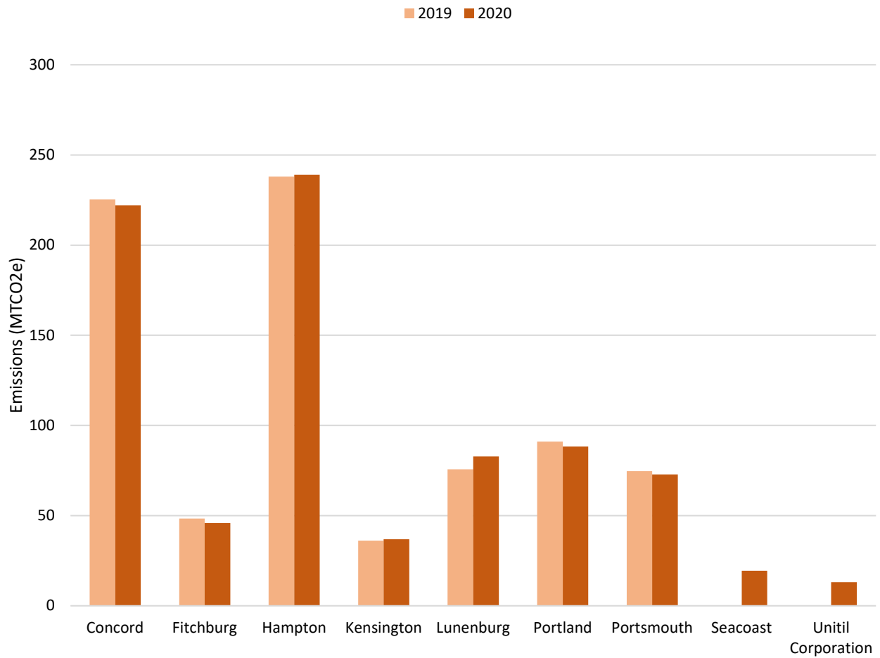
Figure 7: 2019-2020 Emissions from Electricity Use at Company Buildings
