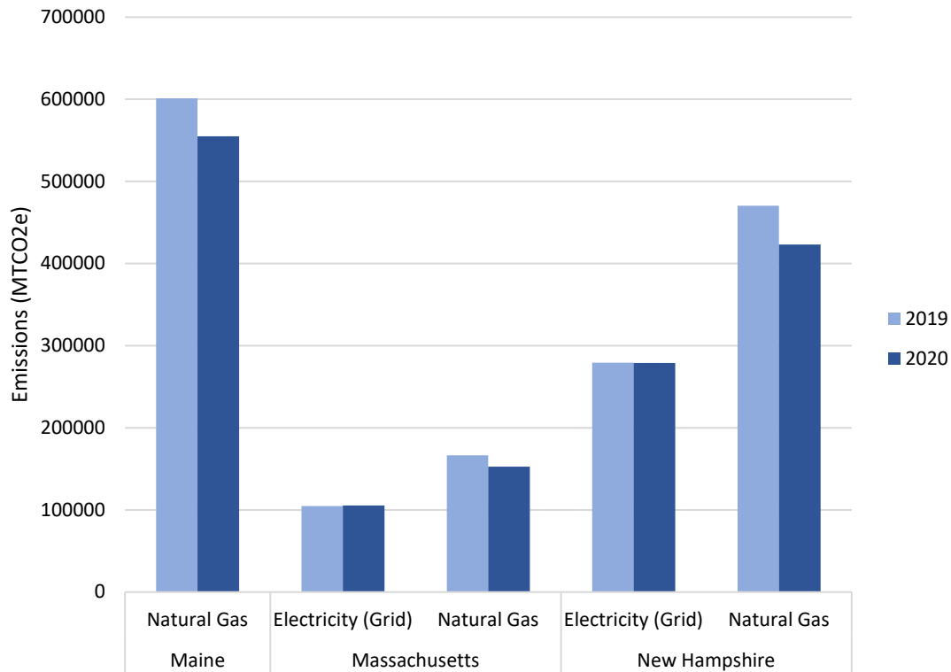
Figure 12: 2019-2020 Emissions from Delivered Energy
