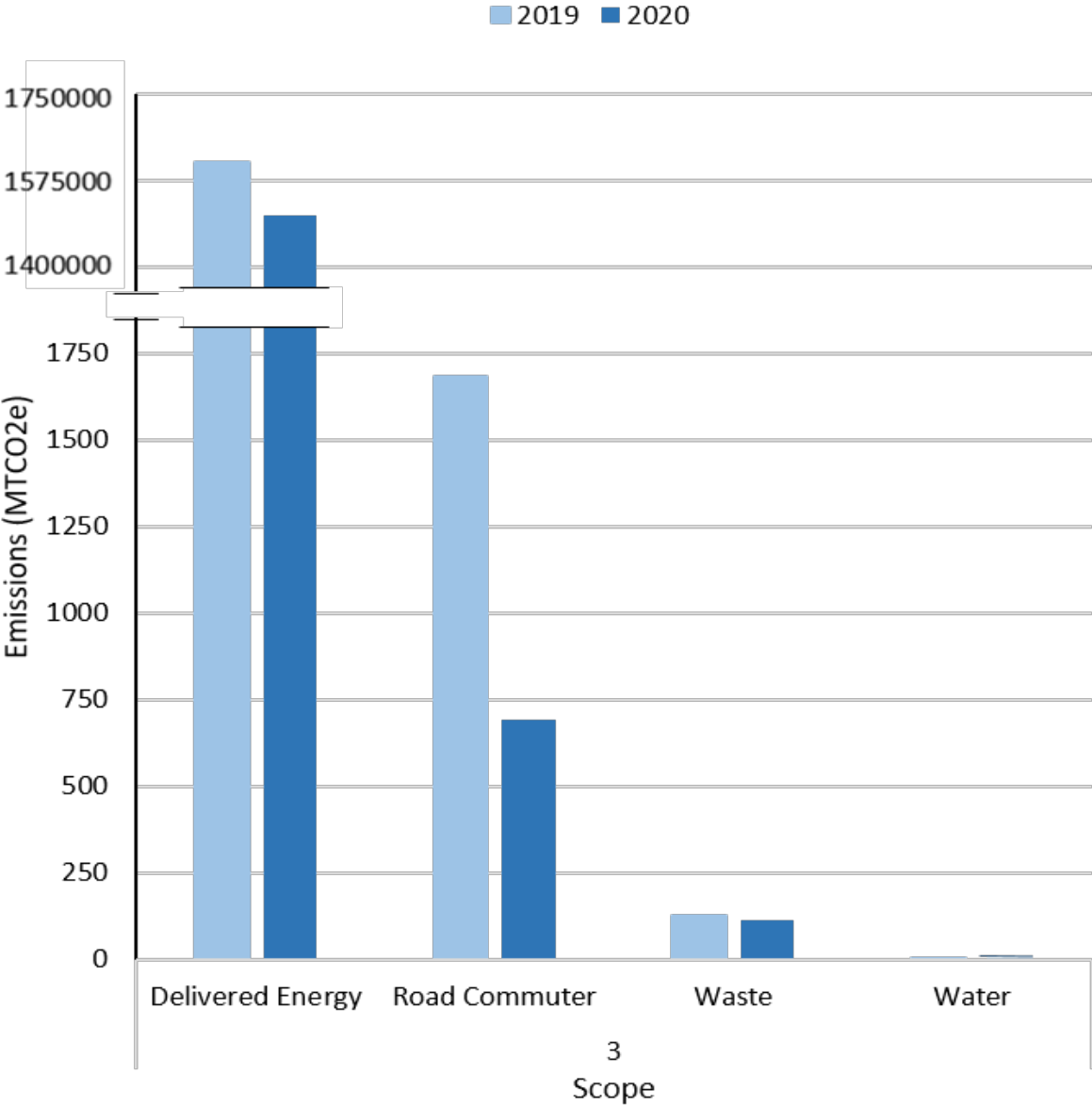
Figure 9: 2019-2020 Scope 3 Summary Chart
